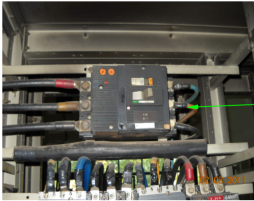
Photo image MCCB
