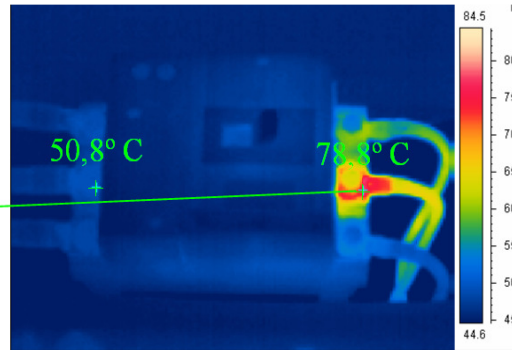
Thermogram of MCCB
